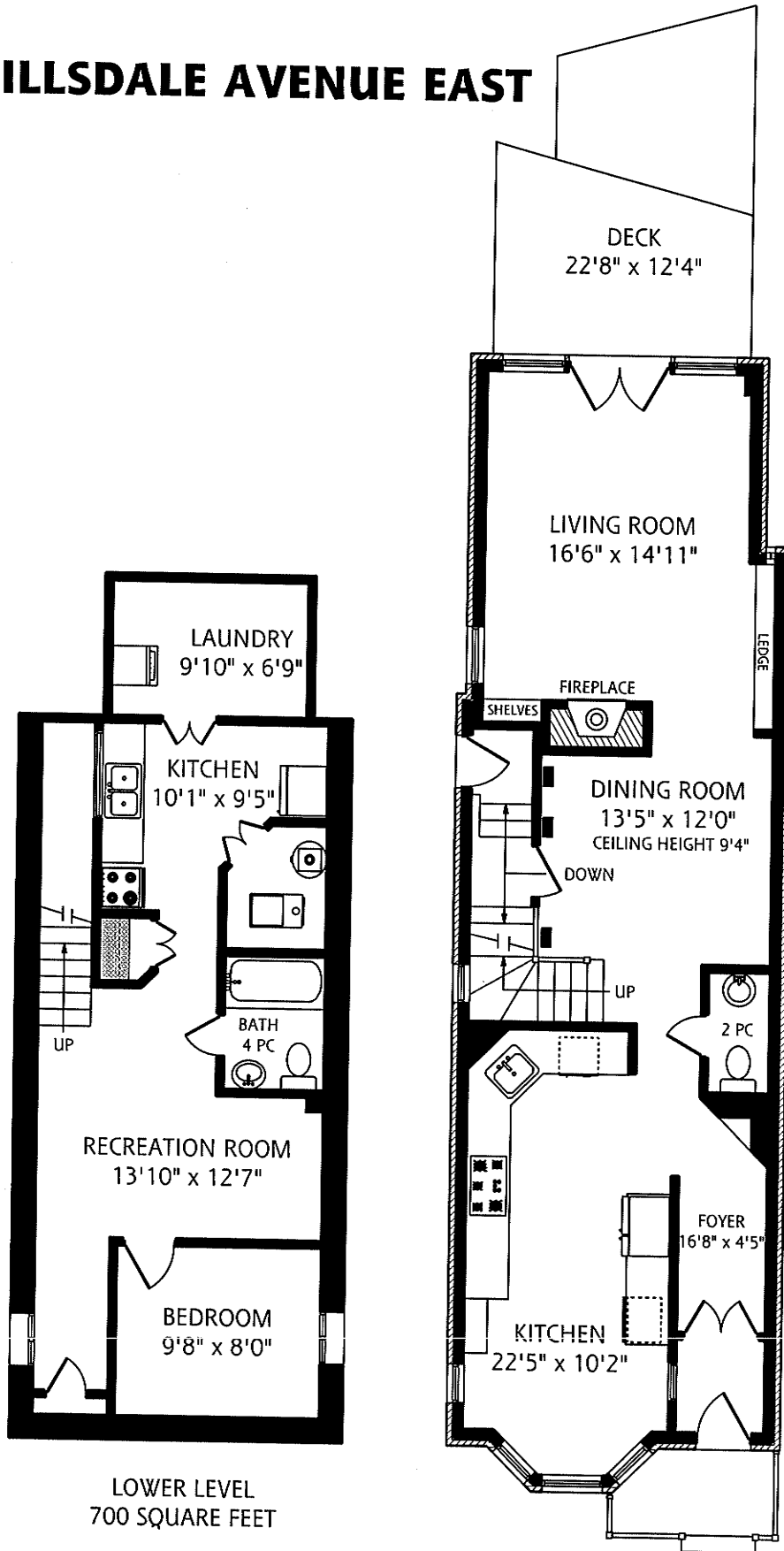
MAIN FLOOR 935 SQUARE FEET
