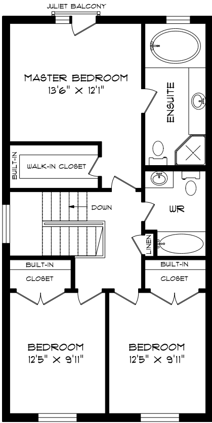
SECOND FLOOR 902 SQUARE FEET
