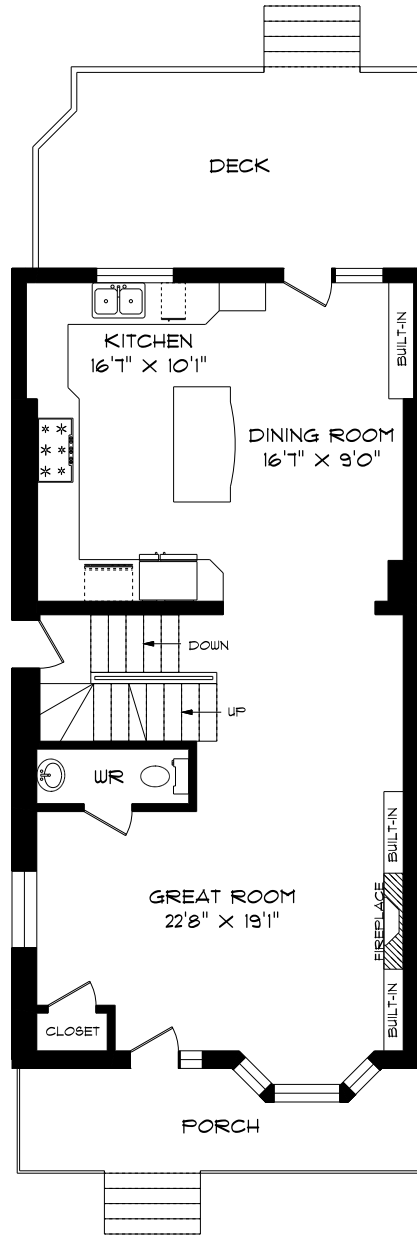
MAIN FLOOR 912 SQUARE FEET
