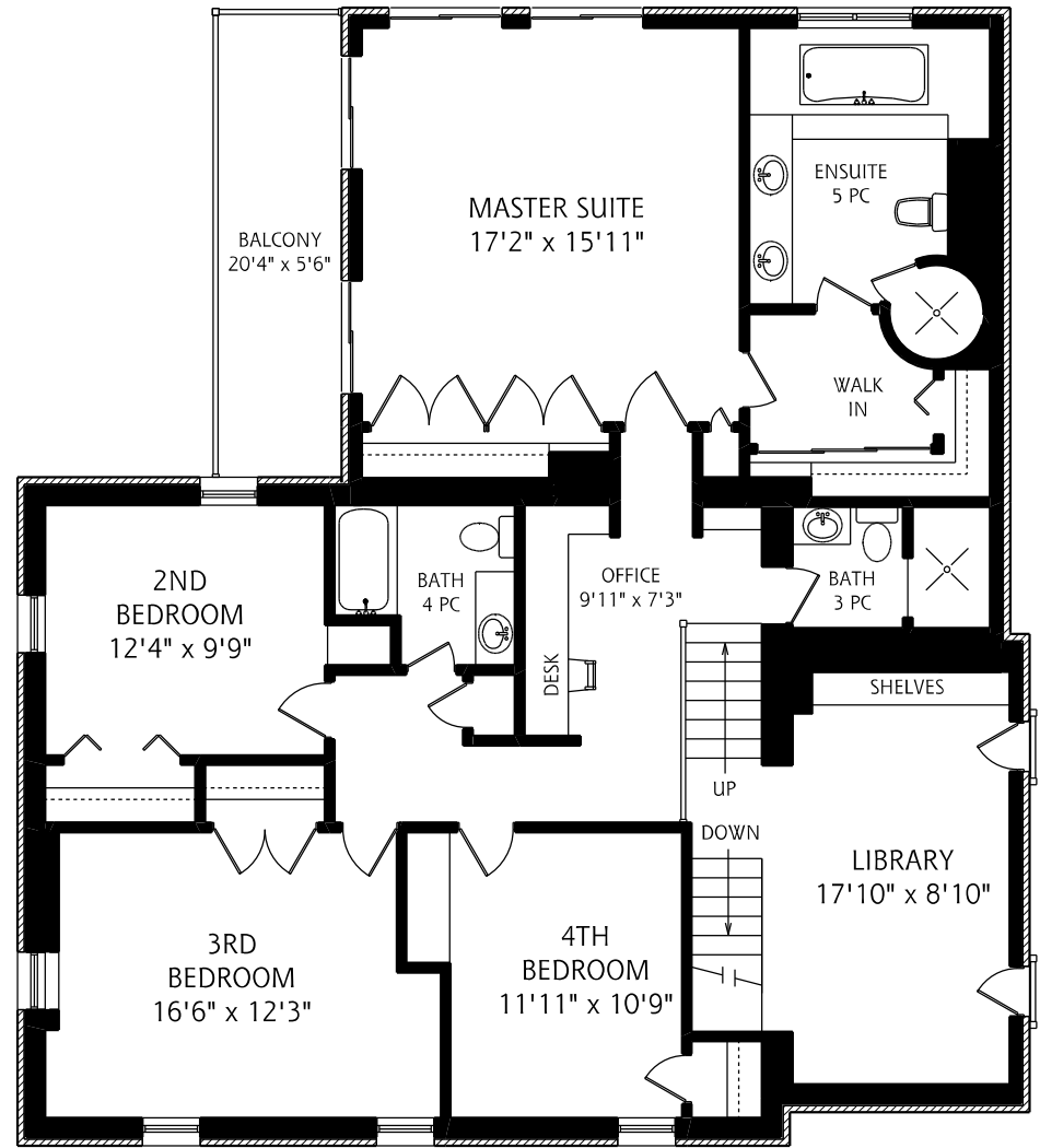
SECOND FLOOR 1,840 SQUARE FEET
